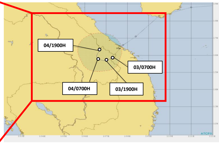
Track of TD KAJIKI by JTWC
